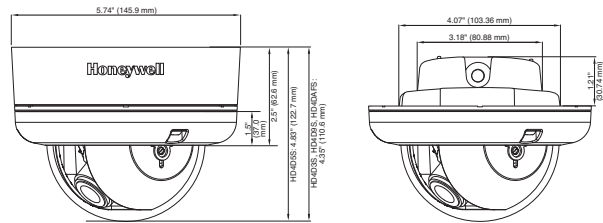
HD4D Series Dimensions
