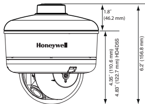
HD4CHIP-PK Pendant Mount
