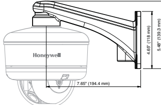
HD4CHIP-WK Wall Mount
